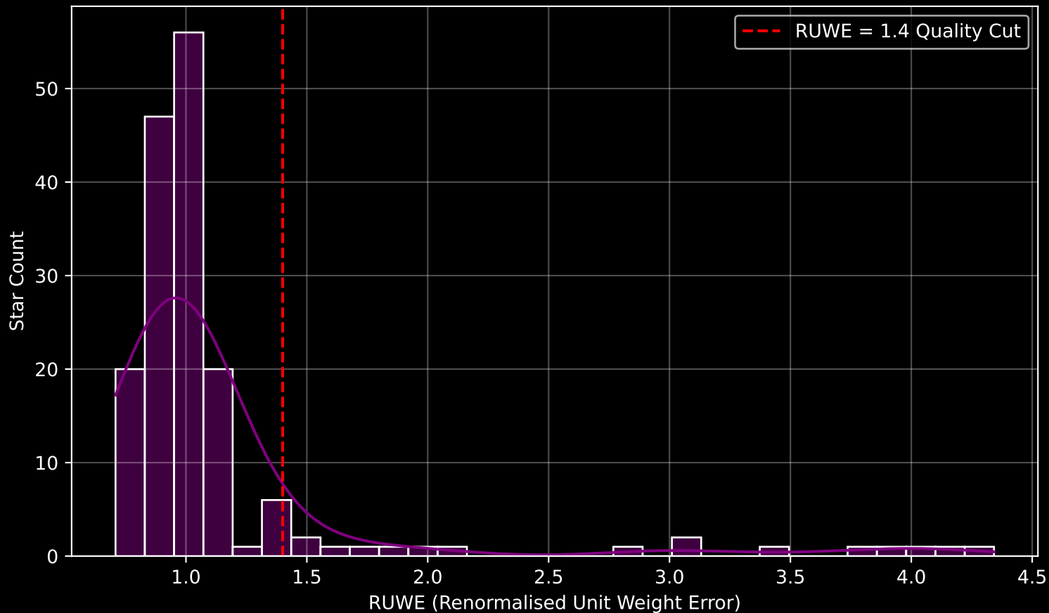
GAPOGEE DR17 Field [CVZTILE_086+27_btx] RUWE Distribution (n= 166)
