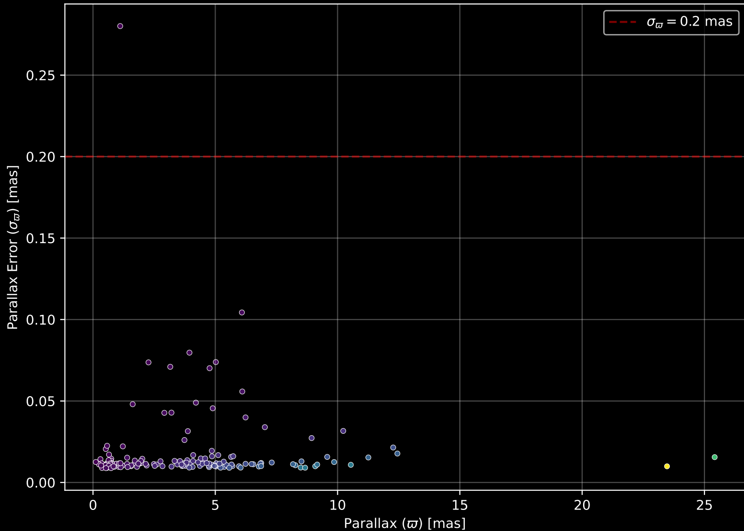
APOGEE DR17 Field: [CVZTILE_086+27_btx] Parallax Quality (n= 173)
