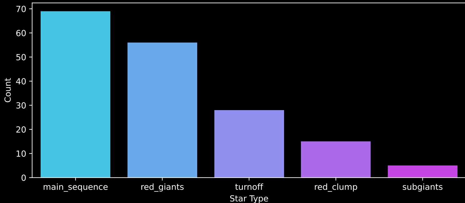
APOGEE DR17 Field: [CVZTILE_086+27_btx] Count plot of Star Type
