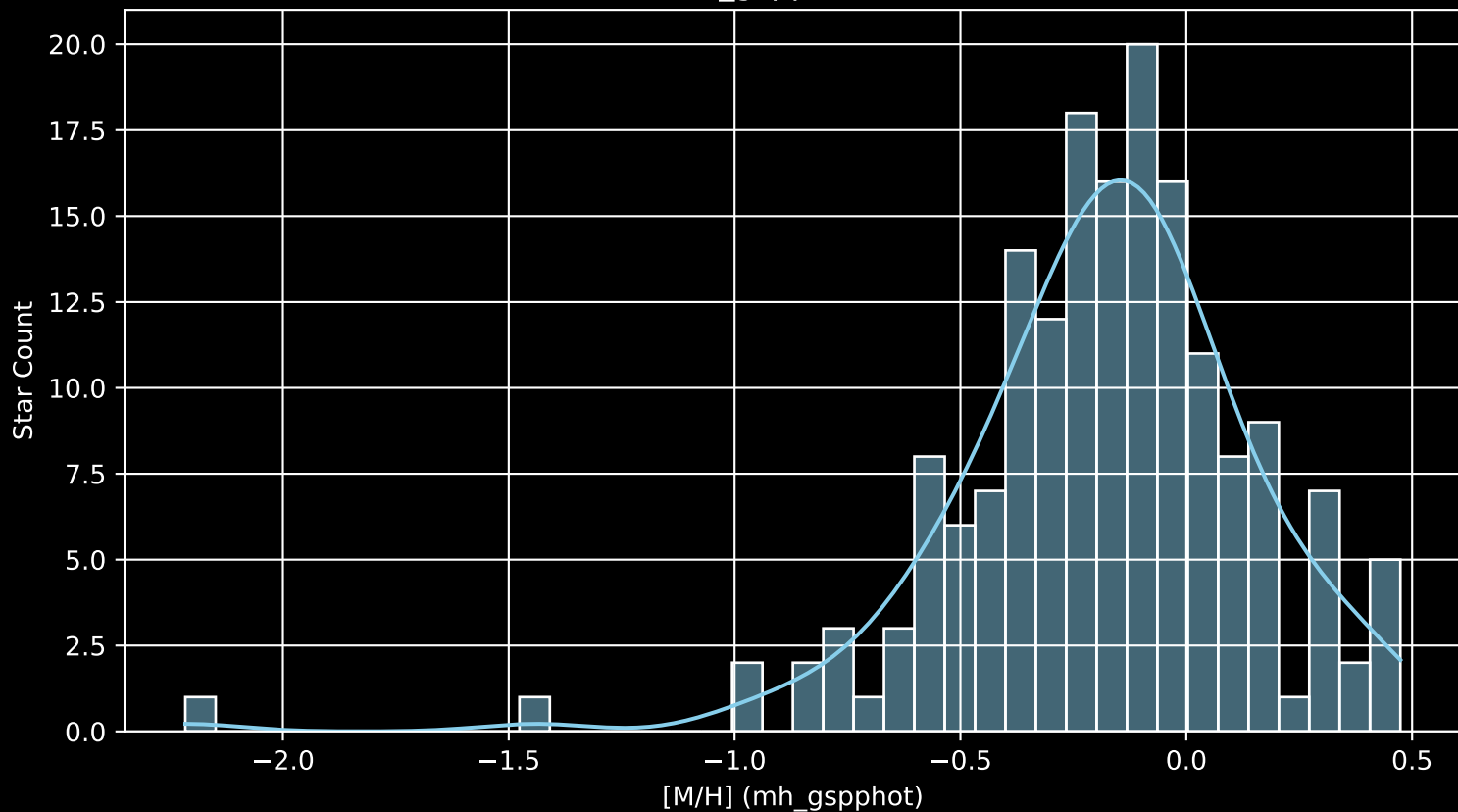
APOGEE DR17 Field: [CVZTILE_086+27_btx [M/H] (mh_gspphot) (n= 173)
