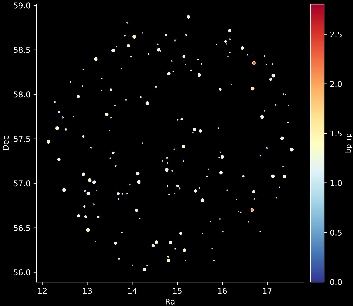
APOGEE DR17 Field: [CVZTILE_086+27_btx] Stars: 173
