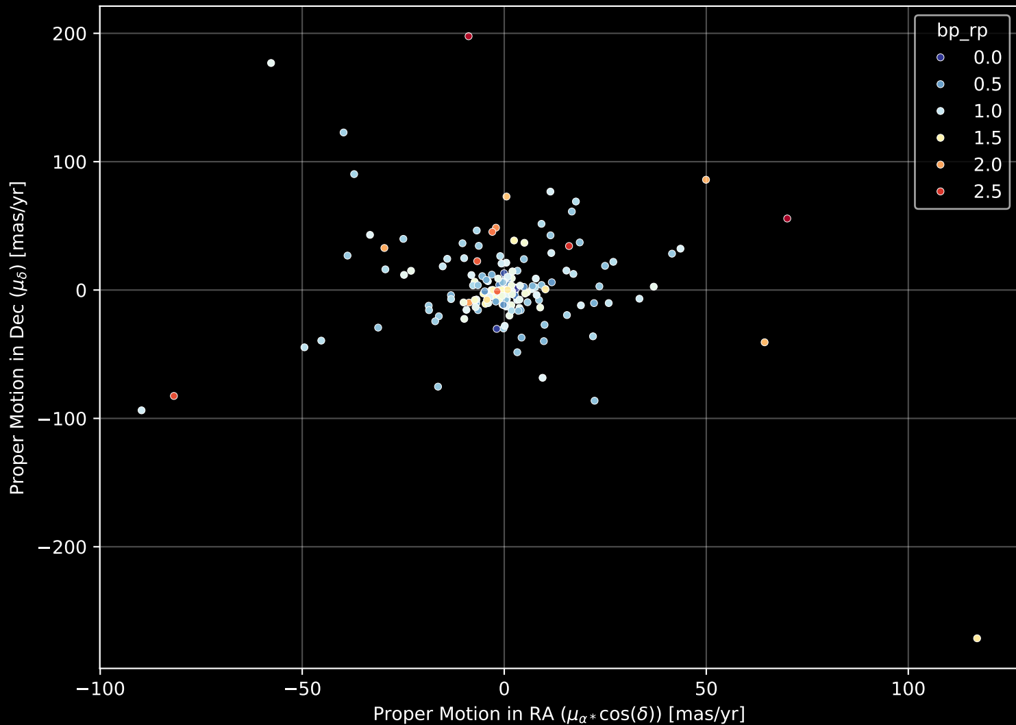
APOGEE DR17 Field: [CVZTILE_086+27_btx] Proper Motion Diagram (n= 173)
